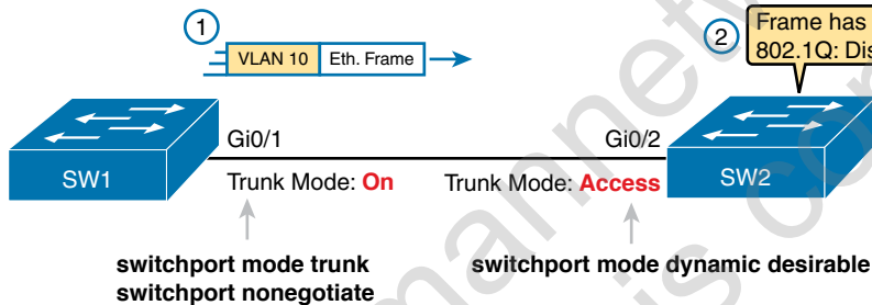
Figure 8-14 Mismatched Trunking Operational States
