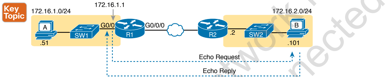
Figure 18-6 Extended Ping Command Tests the Route to 172.16.1.51 (Host A)
