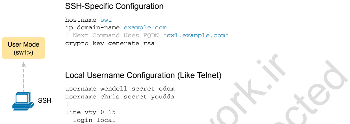
Figure 6-5 Adding SSH Configuration to Local Username Configuration
