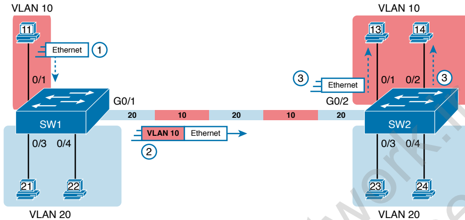
Figure 8-5 VLAN Trunking Between Two Switches
