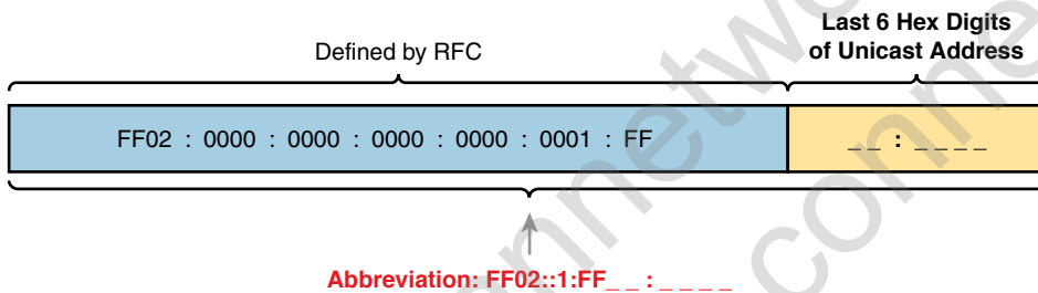
Figure 24-12 Solicited-Node Multicast Address Format
